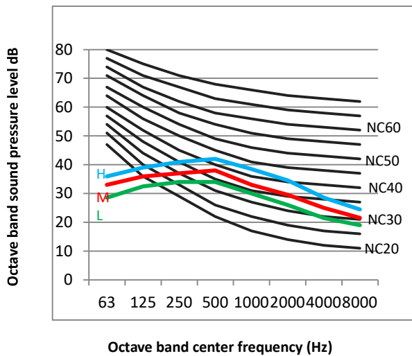
Figure 9.8: BEMP027(31) octave band levels
