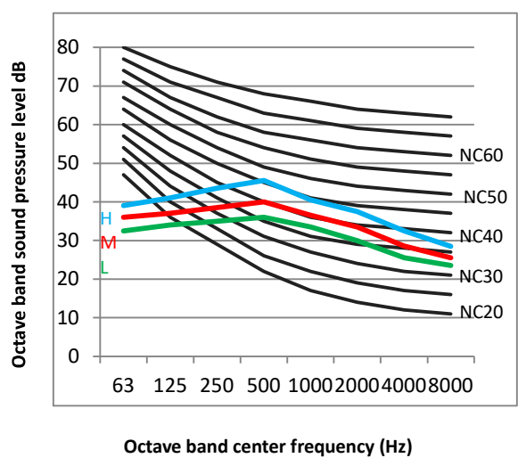
Figure 9.9: BEMP038Q3A-DCM112 octave band levels
