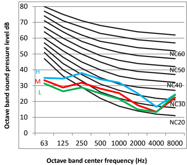
Figure 9.7: BEMP024Q3A-DCM071 octave band levels
