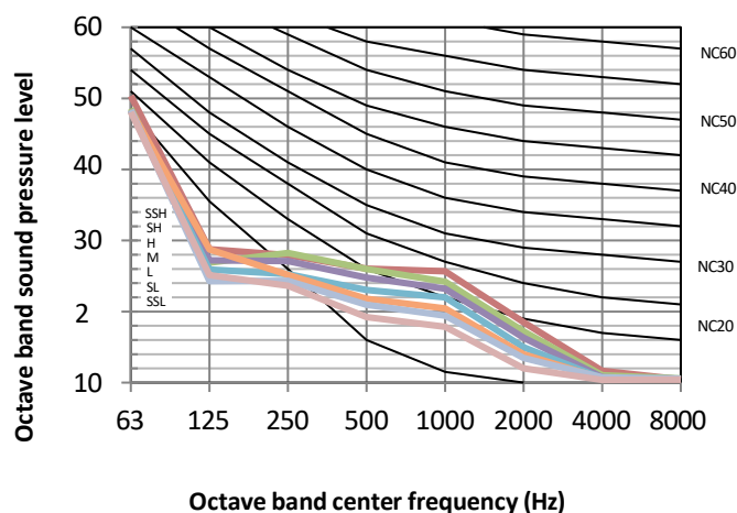
Figure 8.2: BEWM006N0A-DWV018 octave band levels
