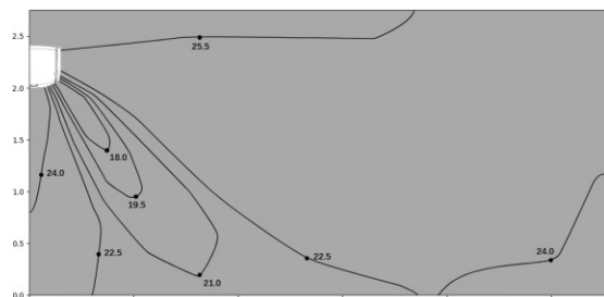
Figure 9.25: BEWM015N0A-DWV045 cooling at 300S
