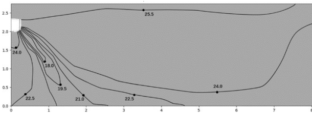
Figure 9.31: BEWM027N0A-DWV080 cooling at 300S
