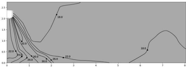
Figure 9.28: BEWM019N0A-DWV056 heating at 300S
