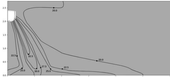
Figure 9.26: BEWM015N0A-DWV045 heating at 300S
