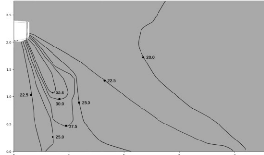
Figure 9.22: BEWM010N0A-DWV028 heating at 300S
