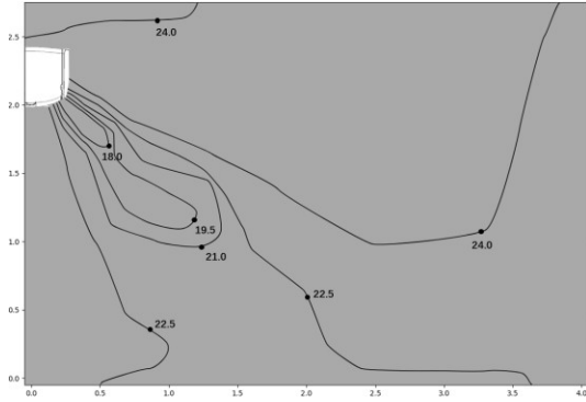
Figure 9.19: BEWM008N0A-DWV022 cooling at 300S
