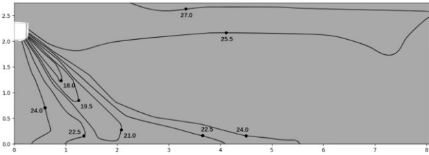
Figure 9.27: BEWM019N0A-DWV056 cooling at 300S
