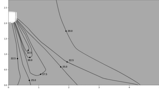
Figure 9.24: BEWM012N0A-DWV036 heating at 300S
