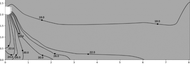
Figure 9.32: BEWM027N0A-DWV080 heating at 300S
