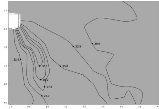
Figure 9.20: BEWM008N0A-DWV022 heating at 300S
