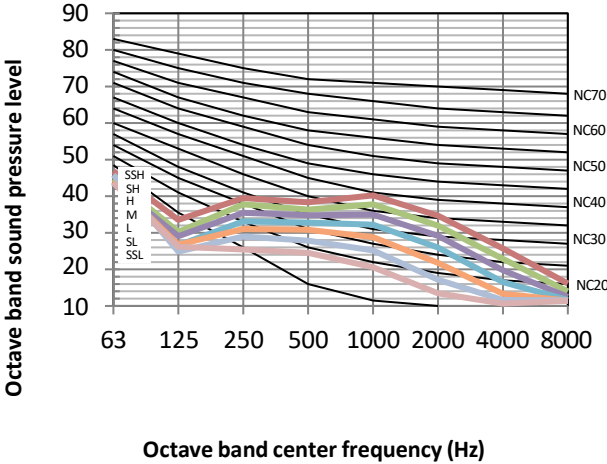
Figure 8.9: BEWM027N0A-DWV080 octave band levels
