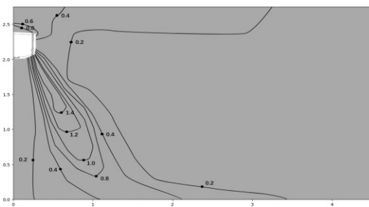
Figure 9.6: BEWM010N0A-DWV028 heating at 300S
