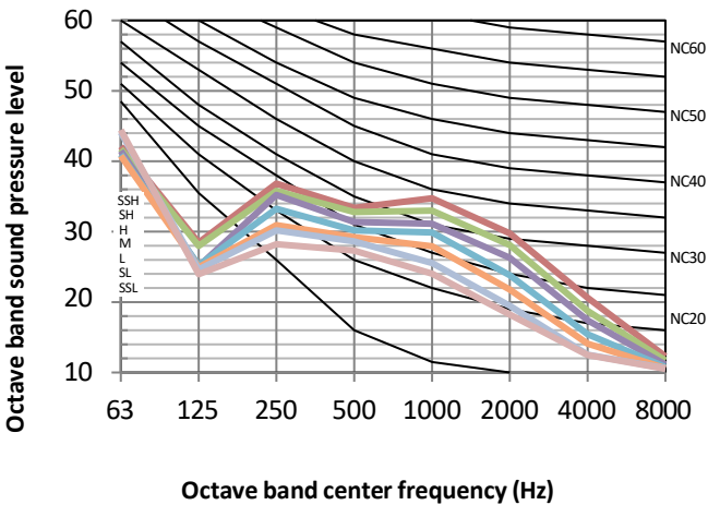
Figure 8.6: BEWM015N0A-DWV045 octave band levels
