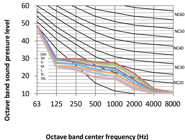
Figure 8.3: BEWM008N0A-DWV022 octave band levels
