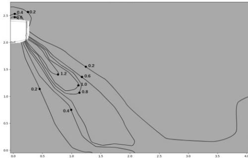
Figure 9.3: BEWM008N0A-DWV022 cooling at 300S
