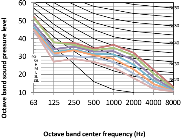
Figure 8.7: BEWM019N0A-DWV056 octave band levels
