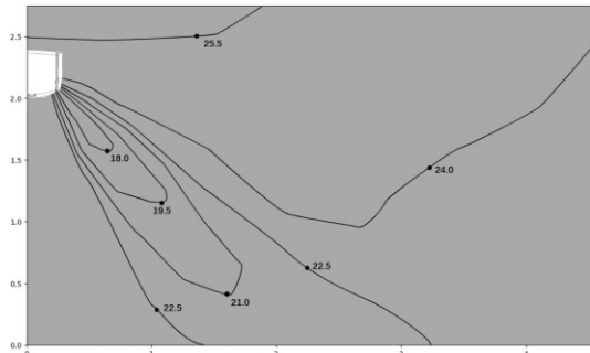
Figure 9.21: BEWM010N0A-DWV028 cooling at 300S
