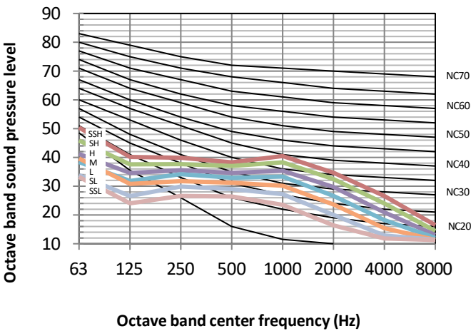
Figure 8.8: BEWM024N0A-DWV071 octave band levels
