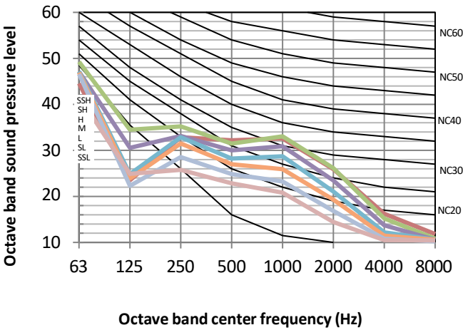
Figure 8.8: BEWM024N0A-DWV071 octave band levels
