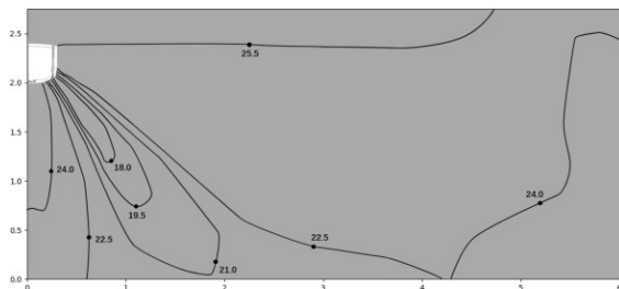
Figure 9.25: BEWM015N0A-DWV045 cooling at 300S
