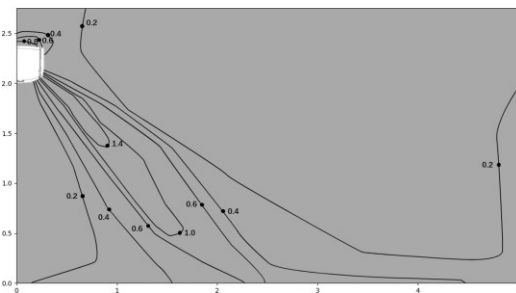
Figure 9.5: BEWM010N0A-DWV028 cooling at 300S
