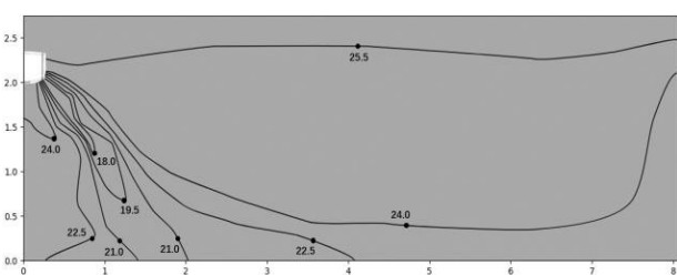
Figure 9.29: BEWM024N0A-DWV071 cooling at 300S
